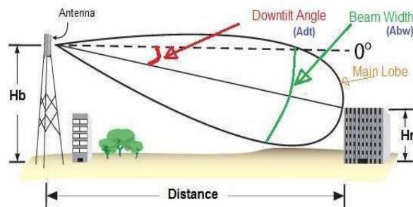
Gambar 3 Tilting Antenna [8]
