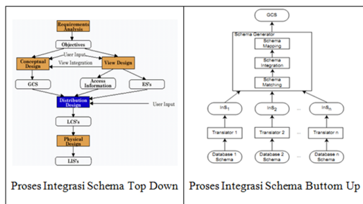
Gambar 2. Mapping Schema
