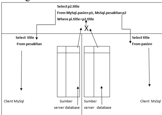
Gambar 12. DML Multidatabase
