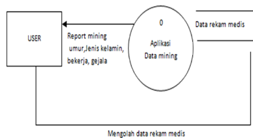
Gambar 1. DFD Level 0
