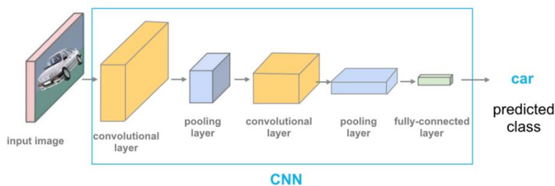
Gambar 3 Contoh Arsitektur Convolutional Neural Network .
