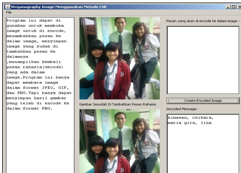
Gambar 6. Extract encoding
