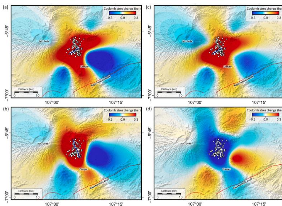
Fig. 5. Modeled Coulomb stress change for four different receiver faults (a) strike-slip fault corresponding to WSW-ENE fault; (b) strike-slip fault corresponding to NNW-SSE fault; (c) strike-slip fault corresponding to the Rajamandala Fault; (d) strike-slip fault corresponding to the Rajamandala Fault. The blue line in each plot denotes the source fault, which corresponds to either the NNW-SSE fault or its conjugate pair. (For interpretation of the references to colour in this figure legend, the reader is referred to the web version of this article.)
