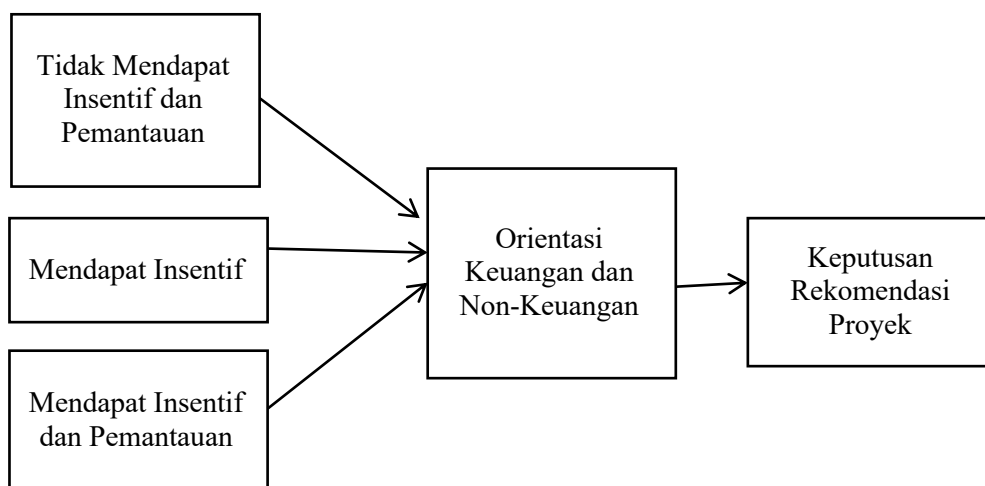
Gambar 1. Model Penelitian
