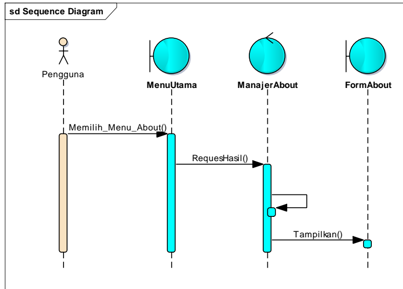
Gambar 5 Sequence Diagram About
