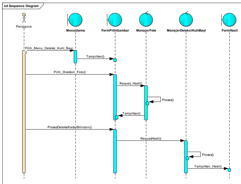
Gambar 4. Sequence Diagram Proses Hasil
