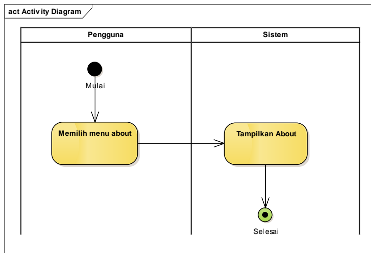
Gambar 3. Activity Diagram About
