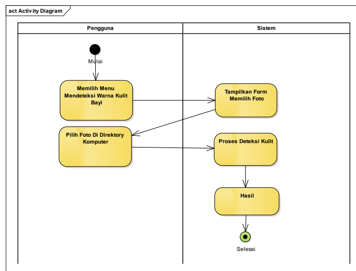
Gambar 2. Activiti Diagram Proses Deteksi
