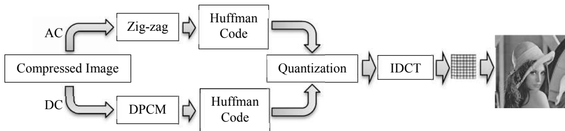
Figure 7. Decoder process on JPEG standard
